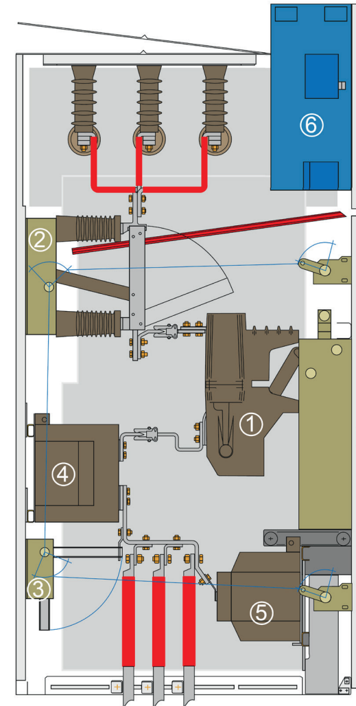
mobile stationary-mounted design W-panel, side view
